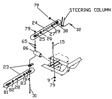
STEERING DETAIL
