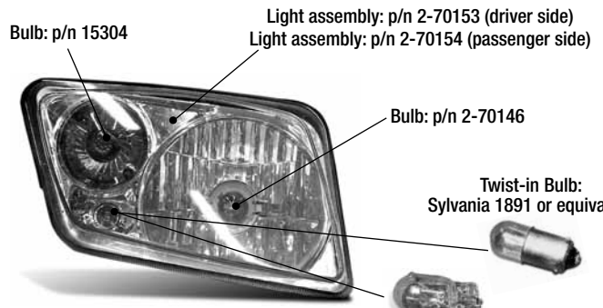
Depending on your year of manufacture, this housing either has a "push-in" or "twist-in" bulb
